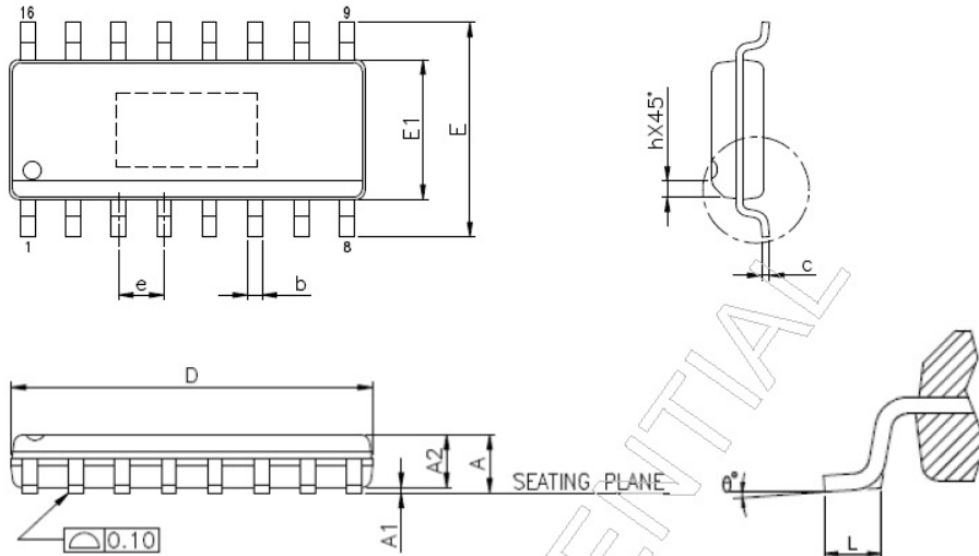
150MIL/SOP-16 PIN
